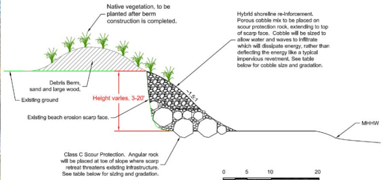
North Scarp Typical Treatment, Section A-A, Scale: 1" = 10'
